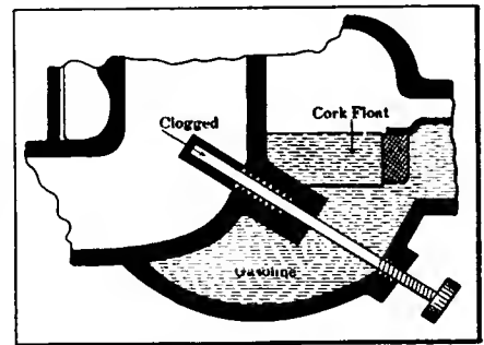
Fig. 4—Section through carbureter, showing needle valve which is apt to clog
